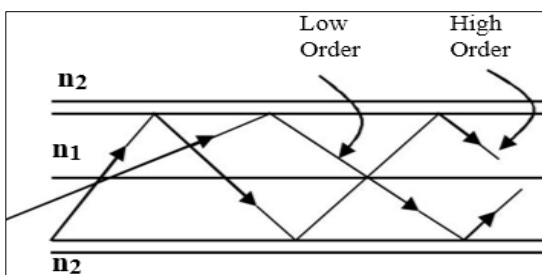
Fig 4: Low and High-order ray paths in a multimode fiber
