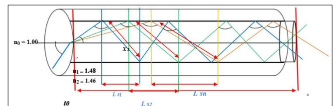
Fig 13: The path of rays in the core of the optical fiber
