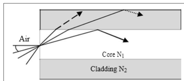
Fig 7: Numerical aperture (NA) properties
