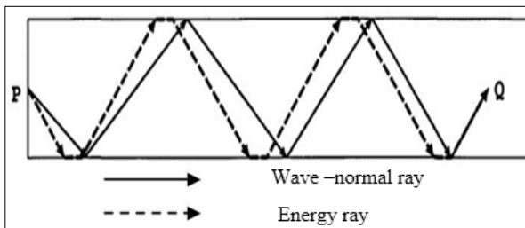
Fig 8: Ray paths in a waveguide.
