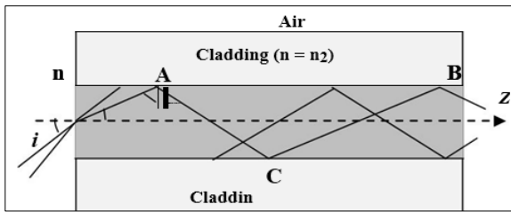
Fig 2: Light rays incident on the core-cladding
