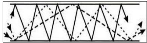
Fig 5: Relatively thick fiber allows many reinforcing angles within the TIR condition
